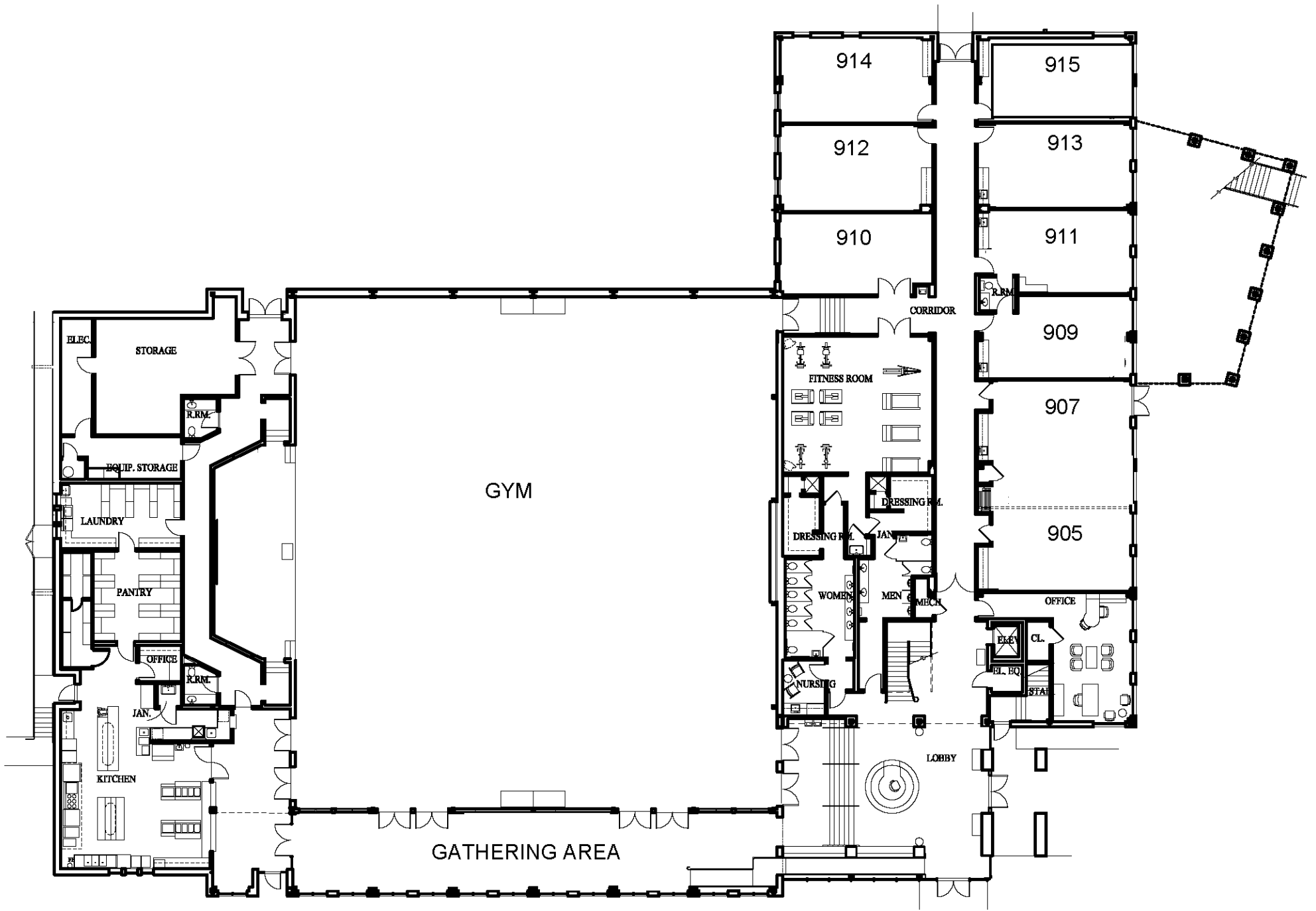
COMMUNITY LIFE CENTER First Floor
